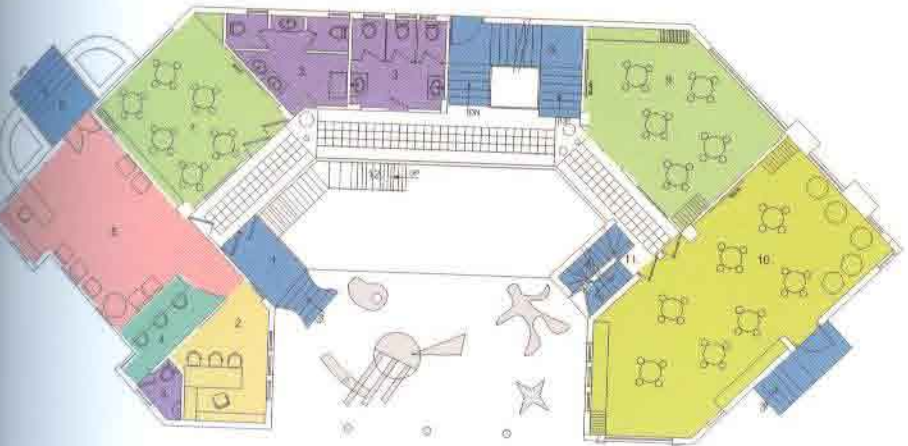
一层平面图 Ground floor plan
